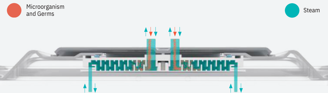
STEAM FILTER CROSS-SECTIONAL VIEW
